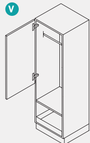
Garderobenschränk Höhe = 1907, 2051, 2195 mm Breite = 600 mm 2 feste Böden 1 Kleiderstange 1 Innenschubkasten Wardrobe Height = 1907, 2051, 2195 mm Width = 600 mm 2 fixed shelves 1 clothes rail 1 internal drawer
